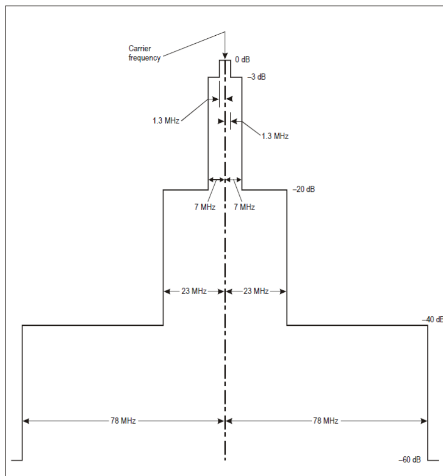
Figure 3-5. Required spectrum limits for transponder transmitter
