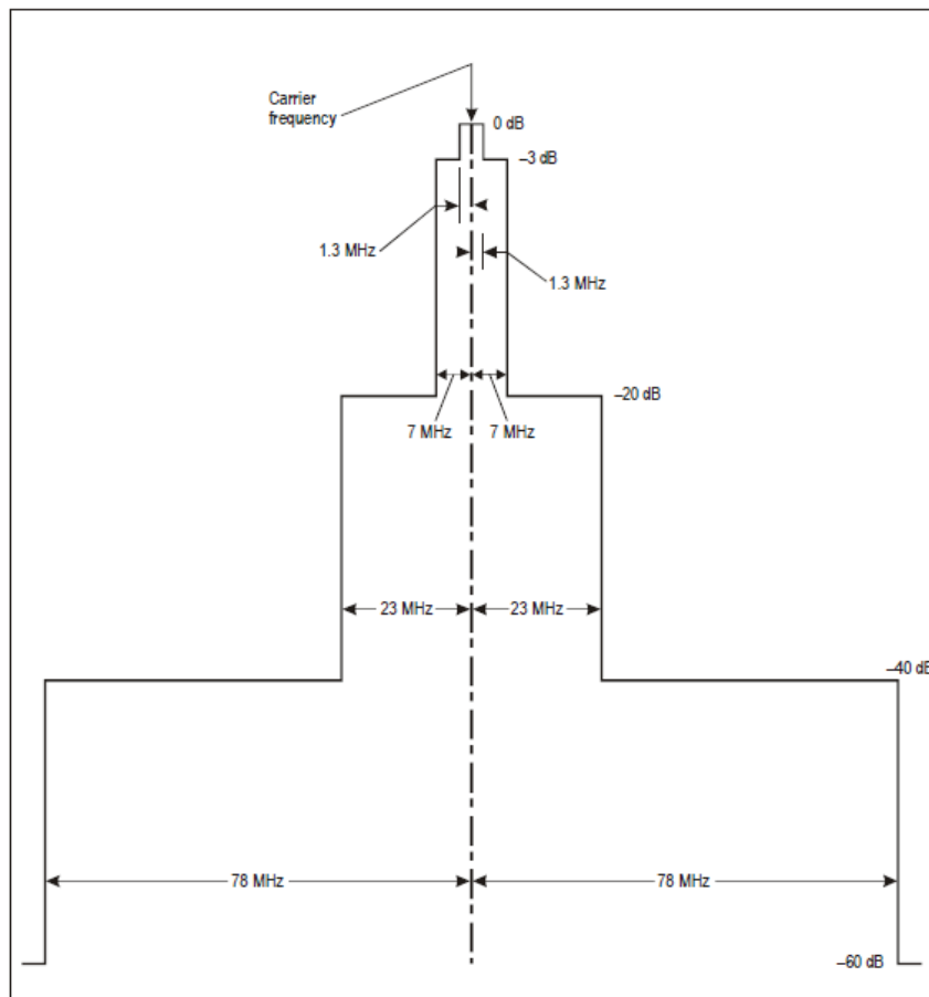
1.5 Figure 1-5: Required spectrum limits for transponder transmitter – Regulation 43
