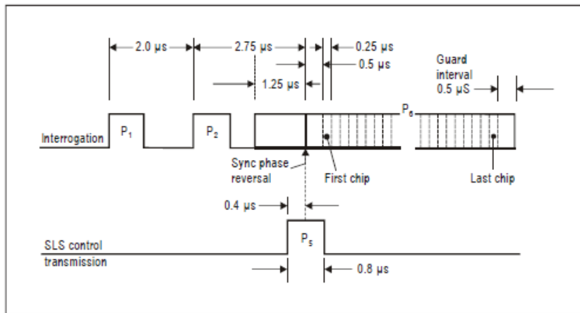
1.4 Figure 1-4: Mode S interrogation pulse sequence (Regulation 42)
